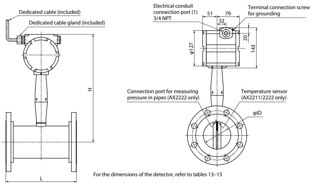
Figure 15. Remote Type, with Flange
