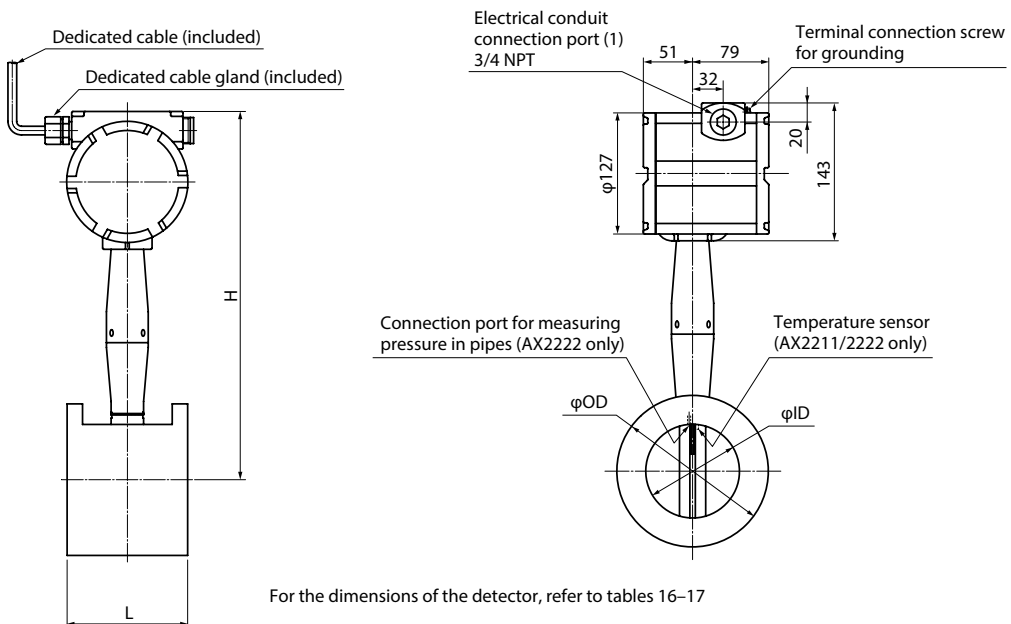
Figure 16. Remote Type, with Wafer <Cable Gland>
