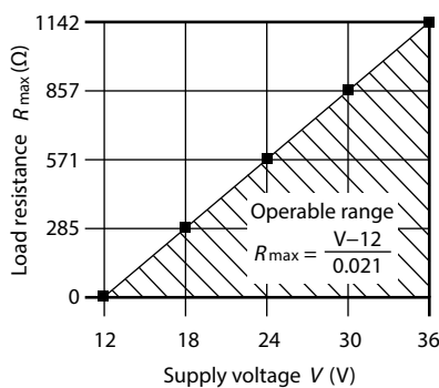
Figure 11. Supply Voltage and Load Resistance of Analog Output
