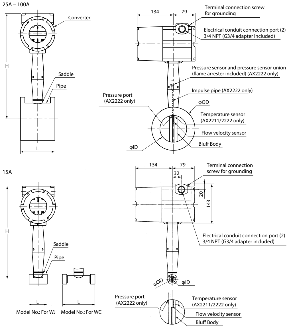
Figure 13. Integral Type, with Wafer
