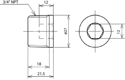
Figure 17. Sealing Plug
