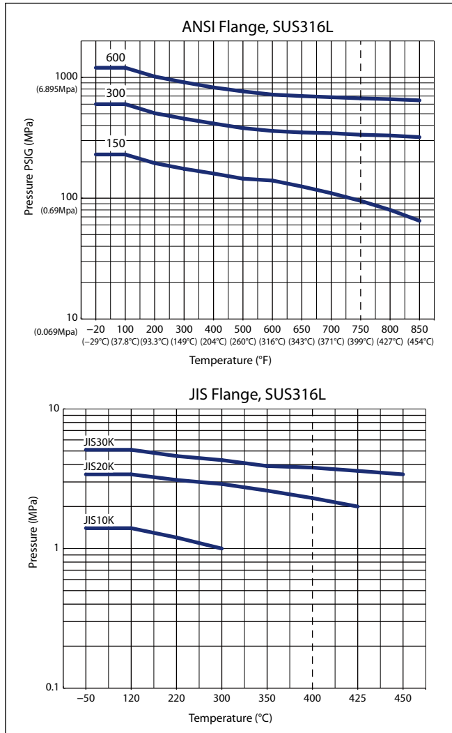
Figure 1. Maximum Operating Pressure
