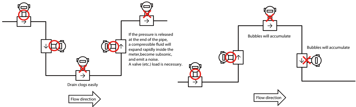
Figure 3. Typical Vortex flowmeter installation
