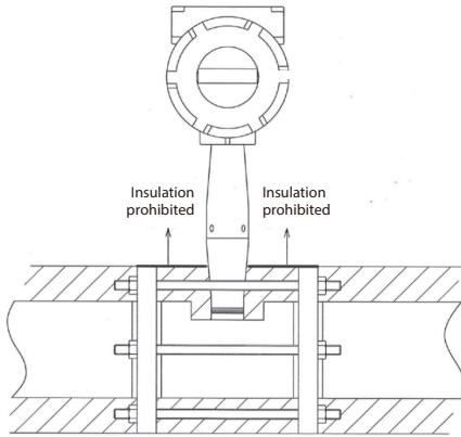
Figure 6. Thermal insulation range for standard and low-temperature models
