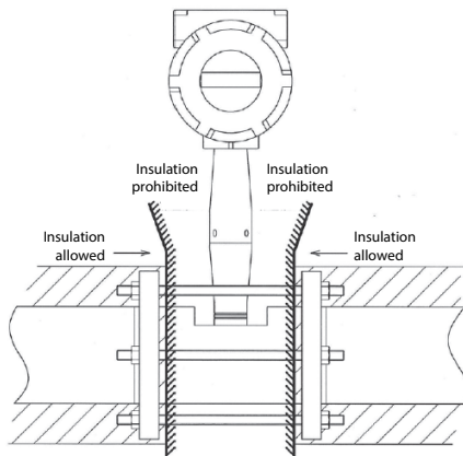
Figure 7. Thermal insulation range for high-temperature models
