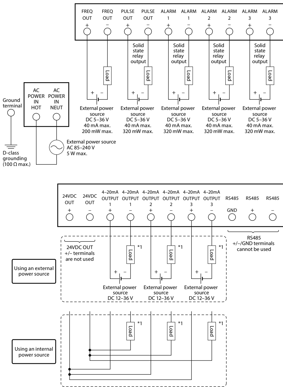
Figure 10. 100 V AC External Power Supply Type Wiring Diagram
