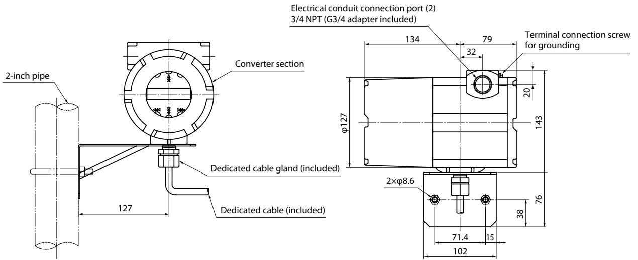
Figure 14. Remote Converter
