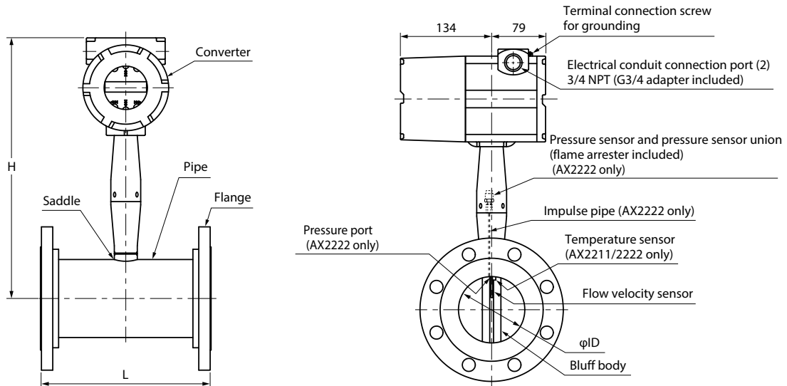
Figure 12. Integral Type, with Flange
